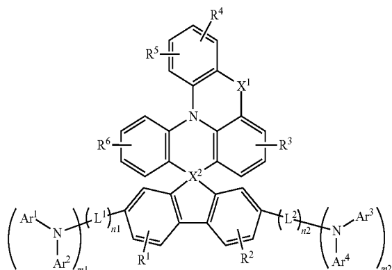
[Chemical Formula 2]
