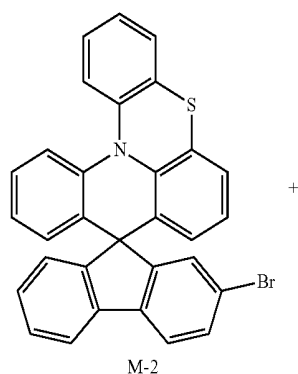
[Reaction Scheme 8]
