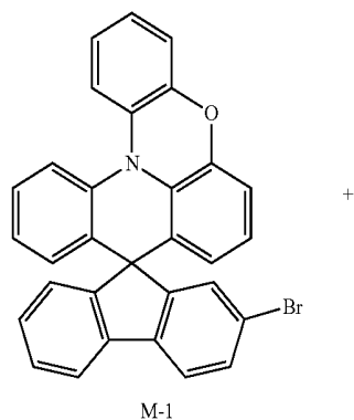
[Reaction Scheme 1]
