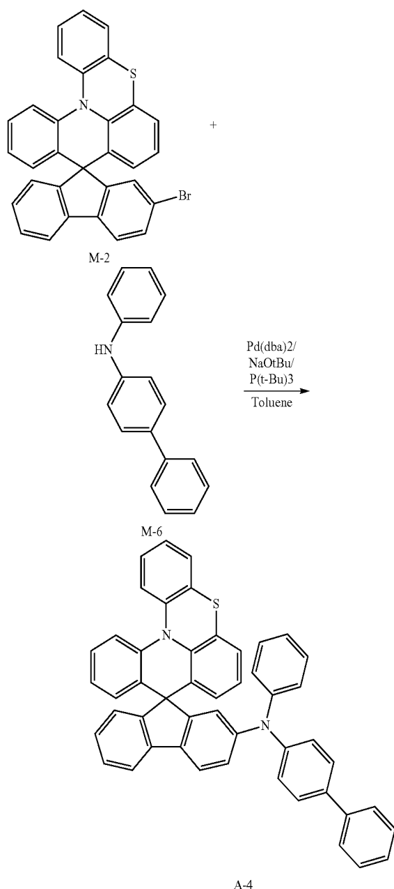
[Reaction Scheme 4]
