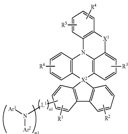
[Chemical Formula 3]
