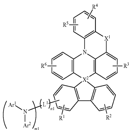
[Chemical Formula 3]
