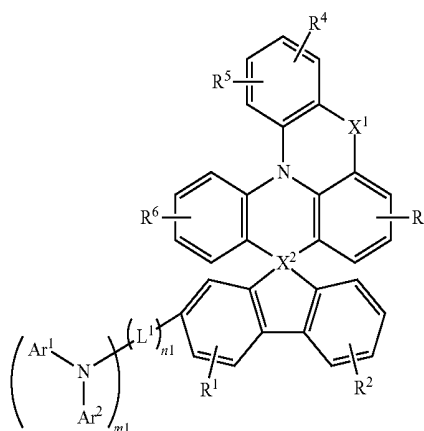
[Chemical Formula 4]
