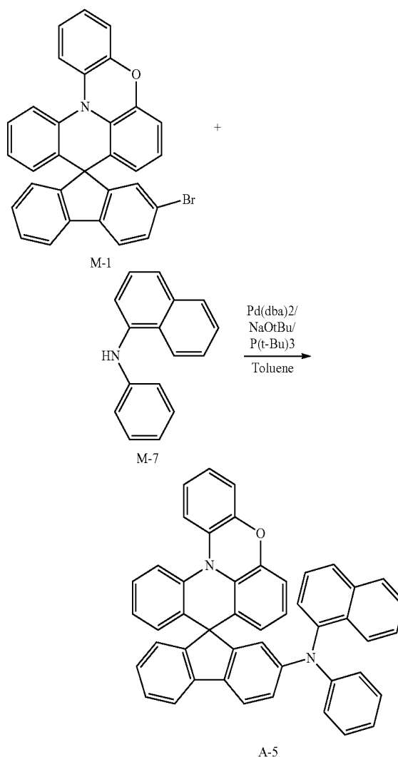
[Reaction Scheme 5]
