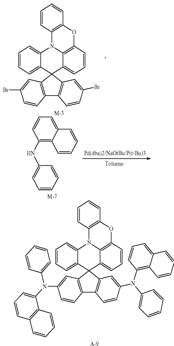
[Reaction Scheme 9]
