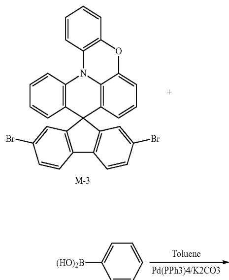
[Reaction Scheme 15]
