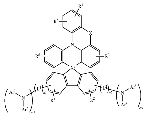
[Chemical Formula 1]
