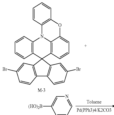
[Reaction Scheme 16]
