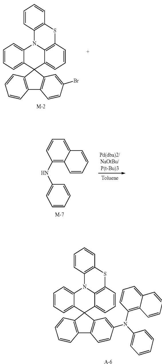
[Reaction Scheme 6]
