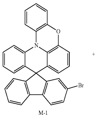
[Reaction Scheme 3]
