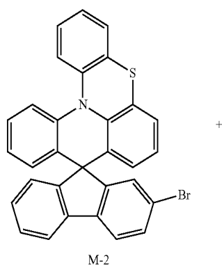
[Reaction Scheme 2]
