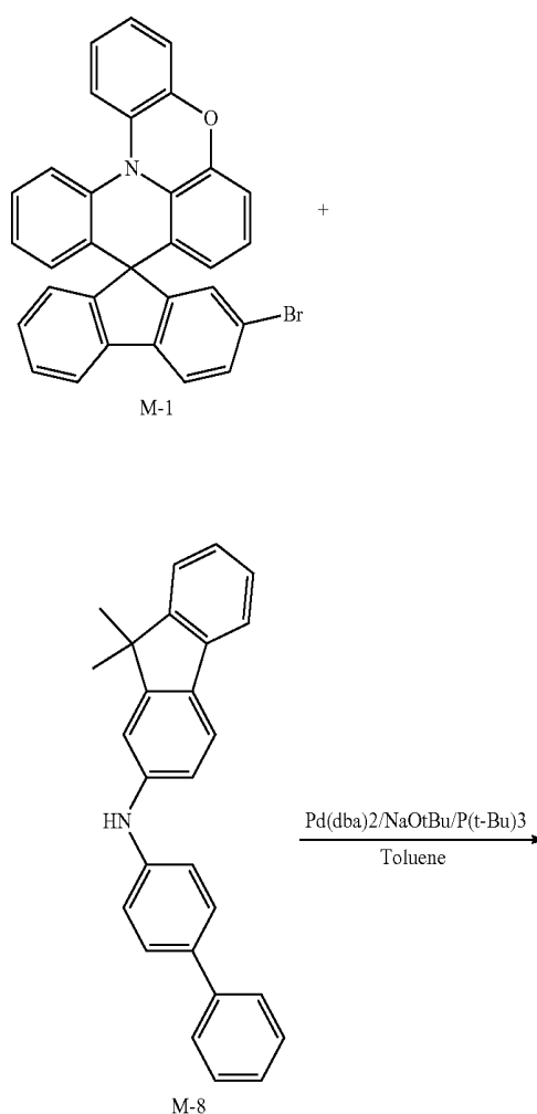
[Reaction Scheme 7]
