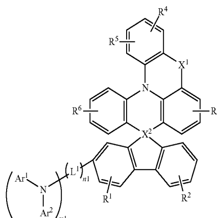
[Chemical Formula 4]
