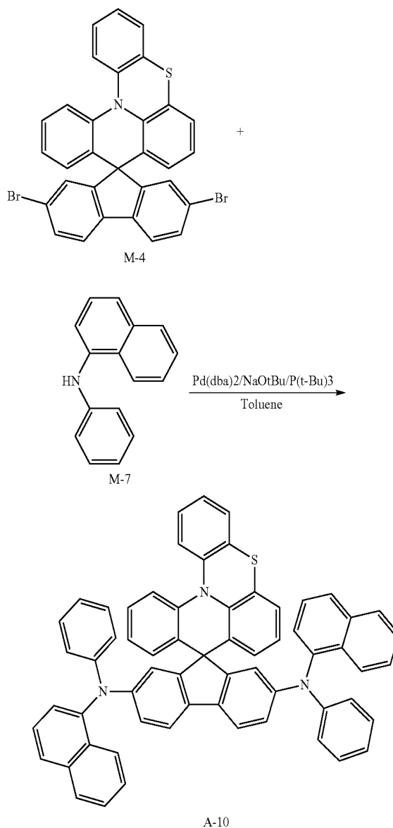
[Reaction Scheme10]
